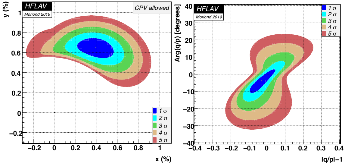
Figure 69.1: Two-dimensional 1\sigma - 5\sigma contours for (x, y) (left) and for (|q/p|, \text{Arg}(q/p)) (right) as obtained by HFLAV [11], from measurements of D^0 \rightarrow K^{(*)}\ell\nu, h^+h^-, K^+\pi^-, K^+\pi^-\pi^0, K^+\pi^-\pi^+\pi^-, K_S^0\pi^+\pi^-, K_S^0K^+K^-, and \pi^+\pi^-\pi^0 decays, and double-tagged branching fractions measured at the \psi(3770) resonance.
