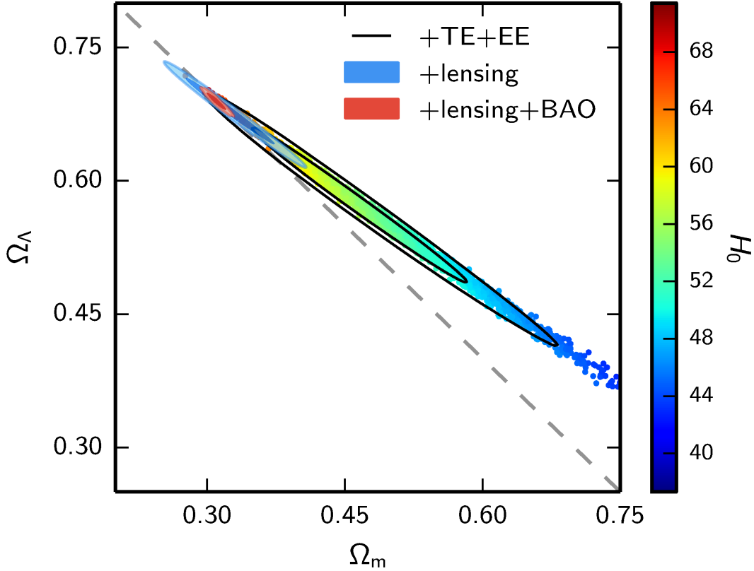
Figure 22.2: Likelihood-based probability densities over the plane \Omega_\Lambda ( i.e. , \Omega_v assuming w = -1 ) vs \Omega_m . The colored locus derives from Planck [33] and shows that the CMB alone requires a flat Universe \Omega_v + \Omega_m \simeq 1 if the Hubble constant is not too high. The SNe Ia results [34] very nearly constrain the orthogonal combination \Omega_v - \Omega_m , and the intersection of these constraints directly favors a flat model with \Omega_m \simeq 0.3 , as does the measurement of the Baryon Acoustic Oscillation lengthscale (for which a joint constraint is shown on this plot). The CMB alone is capable of breaking the degeneracy with H_0 by using the measurements of gravitational lensing that can be made with modern high-resolution CMB data.
