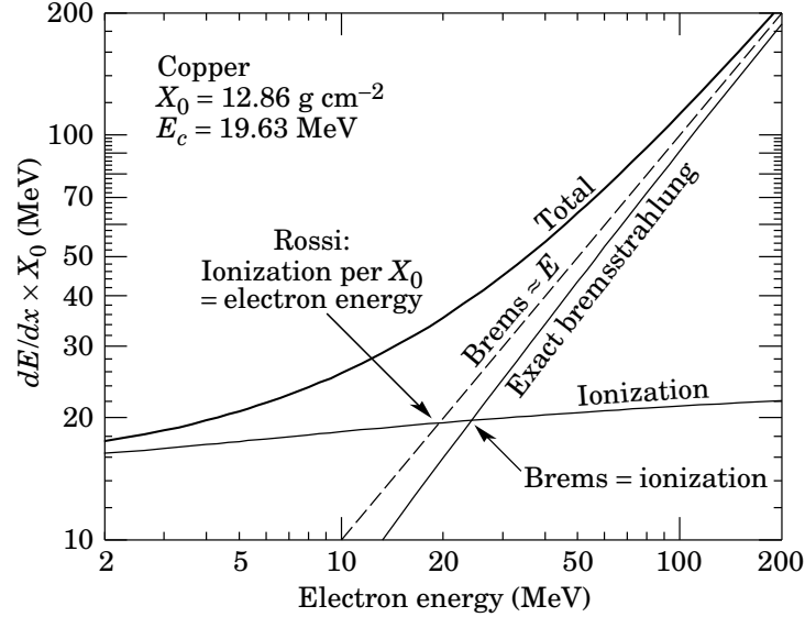
Figure 34.13: Two definitions of the critical energy E_c .
