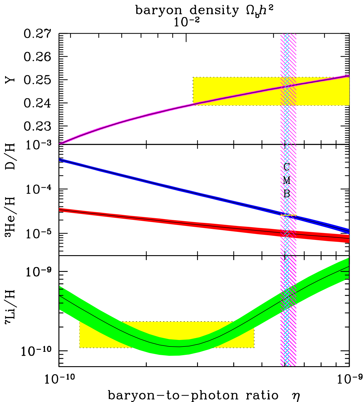
Figure 24.1: The primordial abundances of {}^4\text{He} , D , {}^3\text{He} , and {}^7\text{Li} as predicted by the standard model of Big-Bang nucleosynthesis — the bands show the 95% CL range [5]. Boxes indicate the observed light element abundances. The narrow vertical band indicates the CMB measure of the cosmic baryon density, while the wider band indicates the BBN D+{}^4\text{He} concordance range (both at 95% CL).
