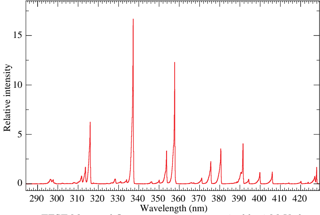
Figure 29.1: TEST Measured fluorescence spectrum excited by 3 MeV electrons in dry air at 800 hPa and 293 K [9].
