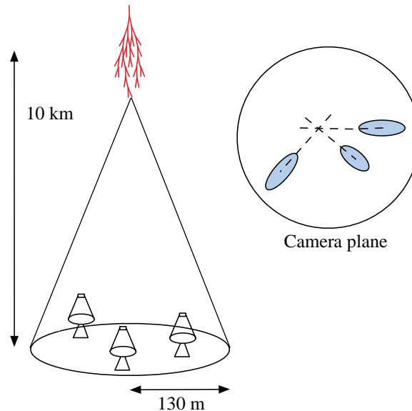
Figure 29.2: A schematic illustration of an atmospheric Cherenkov telescope array. The primary particle initiates an air shower, resulting in a cone of Cherenkov radiation. Telescopes within the Cherenkov light pool record elliptical images; the intersection of the long axes of these images indicates the arrival direction of the primary, and hence the location of a \gamma -ray source in the sky.
