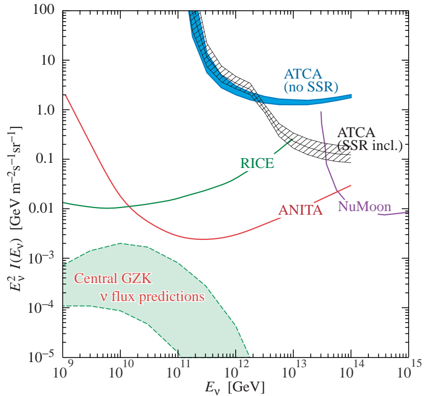
Figure 29.3: Representative \nu flux limits from radio-detection experiments, illustrating the energy ranges for different techniques. Shown are limits from the Rice, ANITA, NuMoon and Lunaska (ATCA) collaborations. NuMoon and Lunaska are low and high frequency lunar scans respectively, showing the strengths of the two different frequency bands. The two separate limits for ATCA are for different models of the lunar regolith; their separation is a measure of the resultant uncertainty. Also shown, for comparison is the mid-range of flux predictions for GZK neutrinos from Ref. 34.
