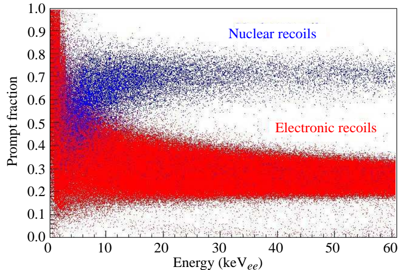
Figure 29.5: An example of pulse-shape discrimination of nuclear recoils and electrons in argon. The prompt fraction is a measure of the pulse shape that clearly separates the two interactions down to very low energy. Figure from Ref. 43.
