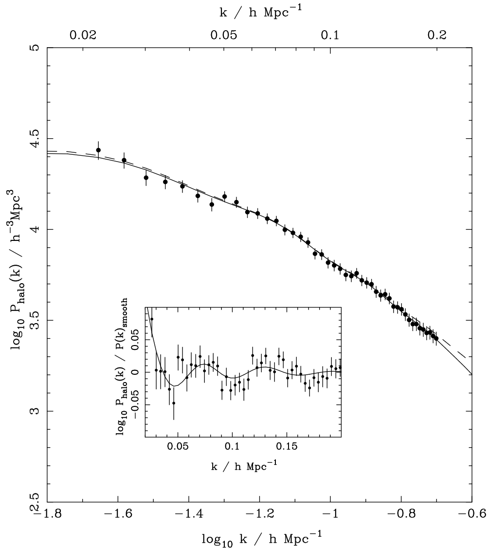
Figure 21.3: The galaxy power spectrum from the SDSS LRGs. The best-fit LRG+WMAP \Lambda CDM model is shown for two sets of nuisance parameters (solid and dashed lines). The BAO inset shows the same data and model divided by a spline fit to the smooth component. [Figure courtesy B. Reid/W. Percival; see Ref. 35.]
