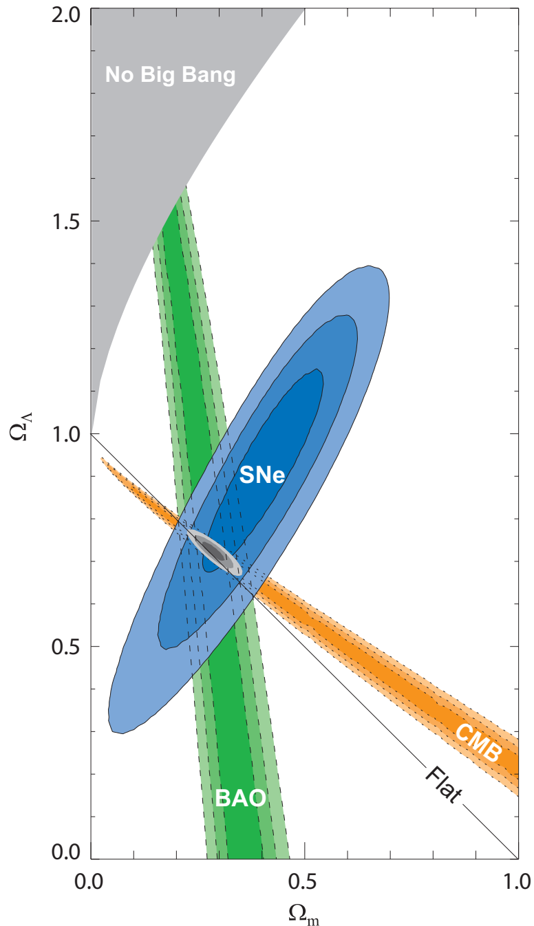
Figure 21.1: Confidence level contours of 68.3%, 95.4% and 99.7% in the \Omega_\Lambda - \Omega_m plane from the CMB, BAOs and the Union SNe Ia set, as well as their combination (assuming w = -1 ). [Courtesy of Kowalski et al. [25]]
