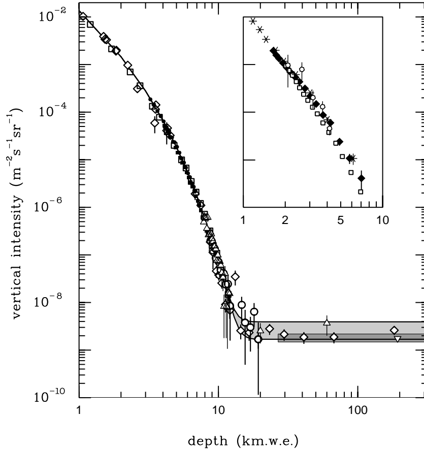
Figure 24.6: Vertical muon intensity vs depth (1 km.w.e. = 10^5 g \text{cm}^{-2} of standard rock). The experimental data are from: \diamond : the compilations of Crouch [58], \square : Baksan [63], \circ : LVD [64], \bullet : MACRO [65], \blacksquare : Frejus [66], and \triangle : SNO [67]. The shaded area at large depths represents neutrino-induced muons of energy above 2 GeV. The upper line is for horizontal neutrino-induced muons, the lower one for vertically upward muons. Darker shading shows the muon flux measured by the SuperKamiokande experiment. The inset shows the vertical intensity curve for water and ice published in Refs. [59–62].
