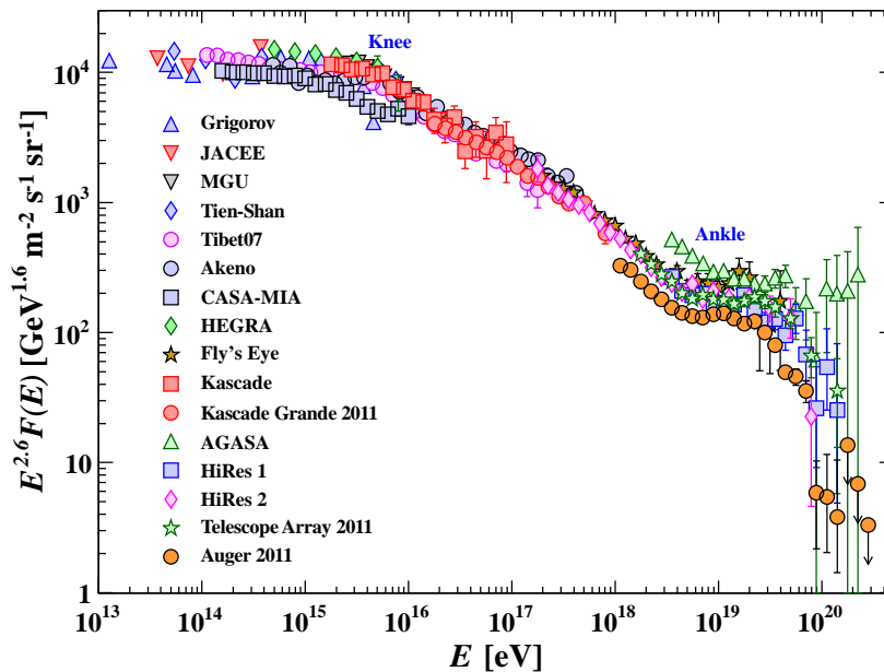
Figure 24.8: The all-particle spectrum as a function of E (energy-per-nucleus) from air shower measurements [79–90,100–104]. Color version at end of book.
