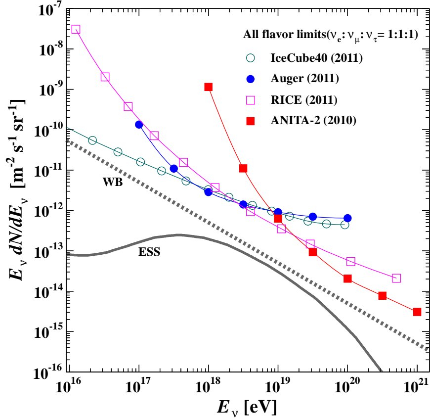
Figure 24.10: Differential limits on the flux of cosmogenic neutrinos set by four neutrino experiments. The curves show the Waxman-Bahcall benchmark flux (WB, [111]) and a representative midrange model for the expected flux of cosmogenic neutrinos (ESS, [110]). The expected flux is uncertain by over an order of magnitude in either direction.
