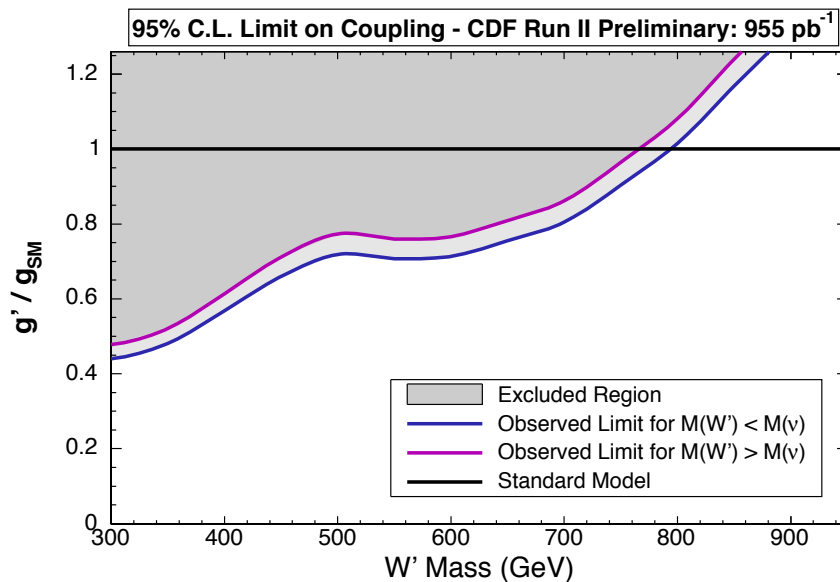
Figure 1: 95% CL exclusion limit from CDF [17] in the gauge coupling versus M_{W'} plane, using the t\bar{b} and \bar{t}b final states. Color version at end of book.
