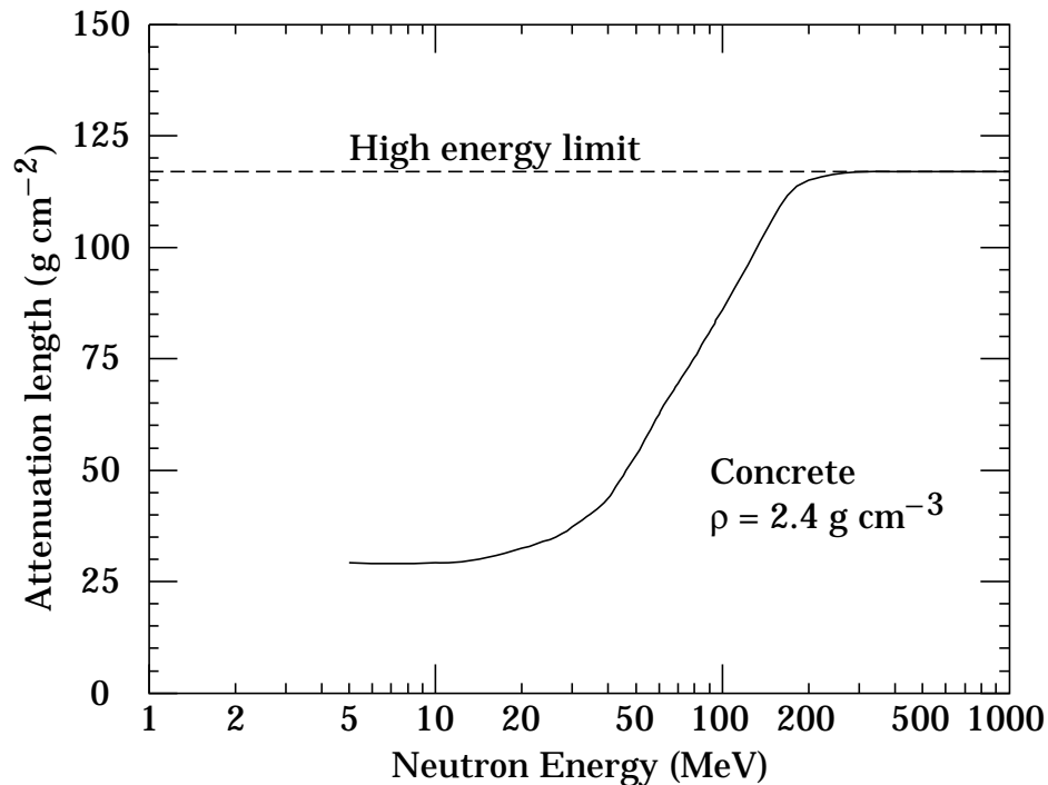
Figure 29.3: The variation of the attenuation length for mono-energetic neutrons in concrete as a function of neutron energy [8].
