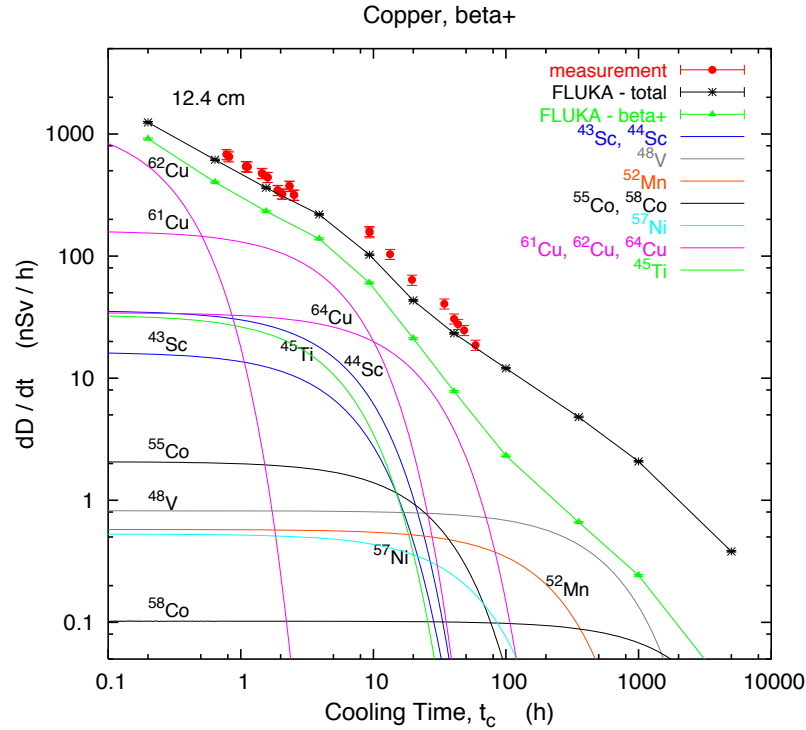
Figure 29.6: Contribution of individual positron-emitting nuclides to the total dose rate at 12.4 cm distance to an activated copper sample [12].
