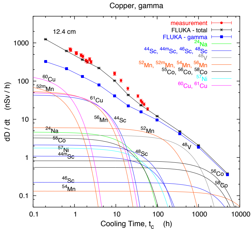
Figure 29.5: Contribution of individual gamma-emitting nuclides to the total dose rate at 12.4 cm distance to an activated copper sample [12].
