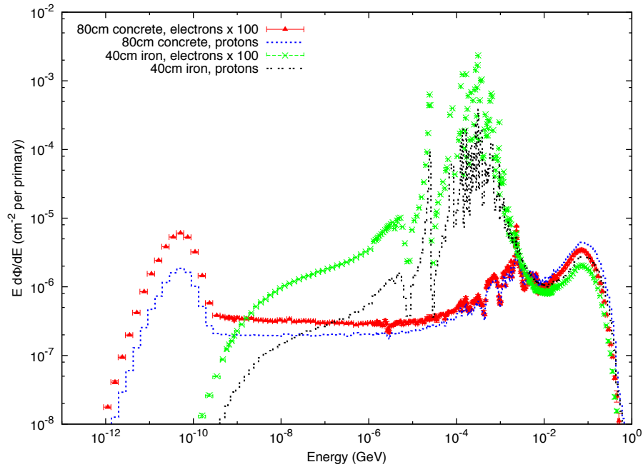
Figure 29.2: Neutron energy spectra calculated with the FLUKA code [6,7] from 25 GeV proton and electron beams on a thick copper target. Spectra are evaluated at 90^\circ to the beam direction behind 80 cm of concrete or 40 cm of iron. All spectra are normalized per beam particle. In addition, spectra for electron beam are multiplied by a factor of 100.
