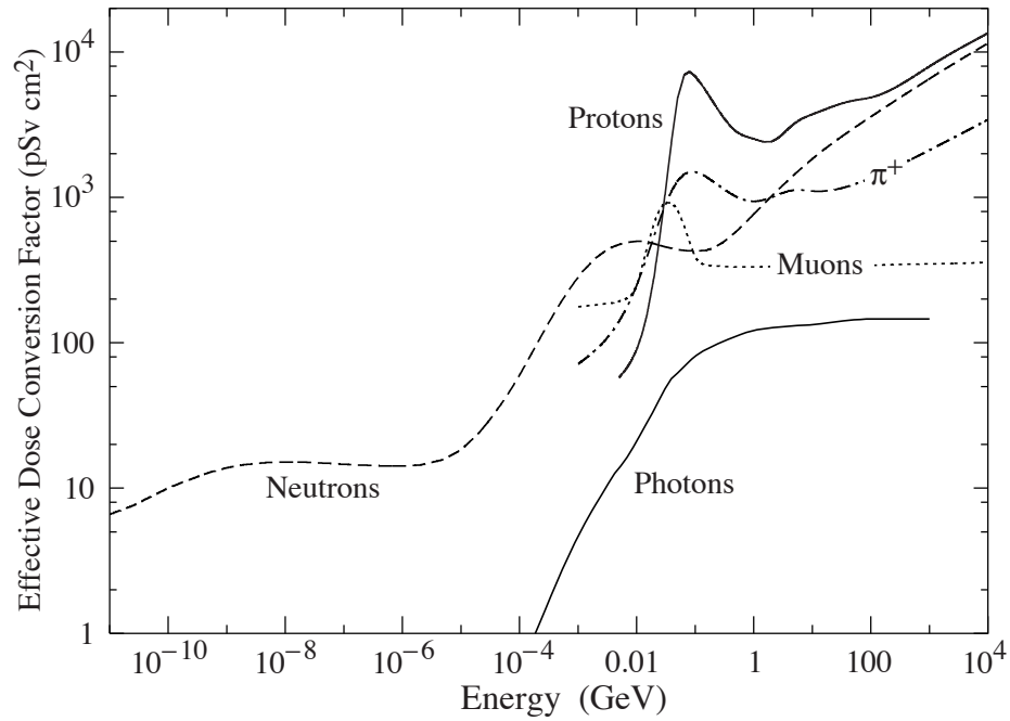
Figure 29.4: Fluence to effective dose conversion coefficients for anterior-posterior irradiation and various particles [11].
