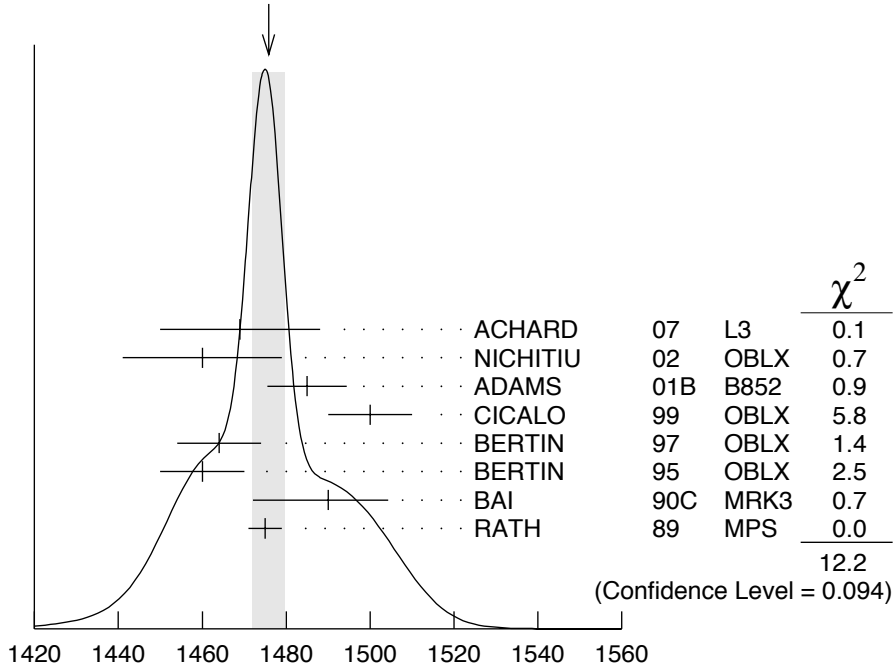
\eta(1475) mass, K\bar{K}\pi mode ( K^*(892) K dominant) (MeV)
