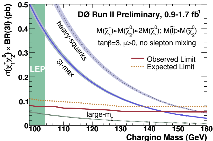
Figure 6: Upper limit from DØ on the product of cross section times branching ratio into three leptons for the associated \tilde{\chi}^{\pm}_1 \tilde{\chi}^0_2 production at the Tevatron. The “3l-max” theoretical curve corresponds to the hypotheses detailed in the text. See full-color version on color pages at end of book.
