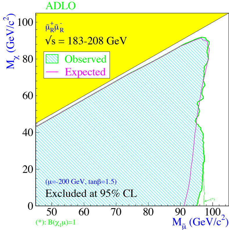
Figure 1: Region in the (m_{\tilde{\mu}_R}, m_{\tilde{\chi}_1^0}) plane excluded by the searches for smuons at LEP. See full-color version on color pages at end of book.
