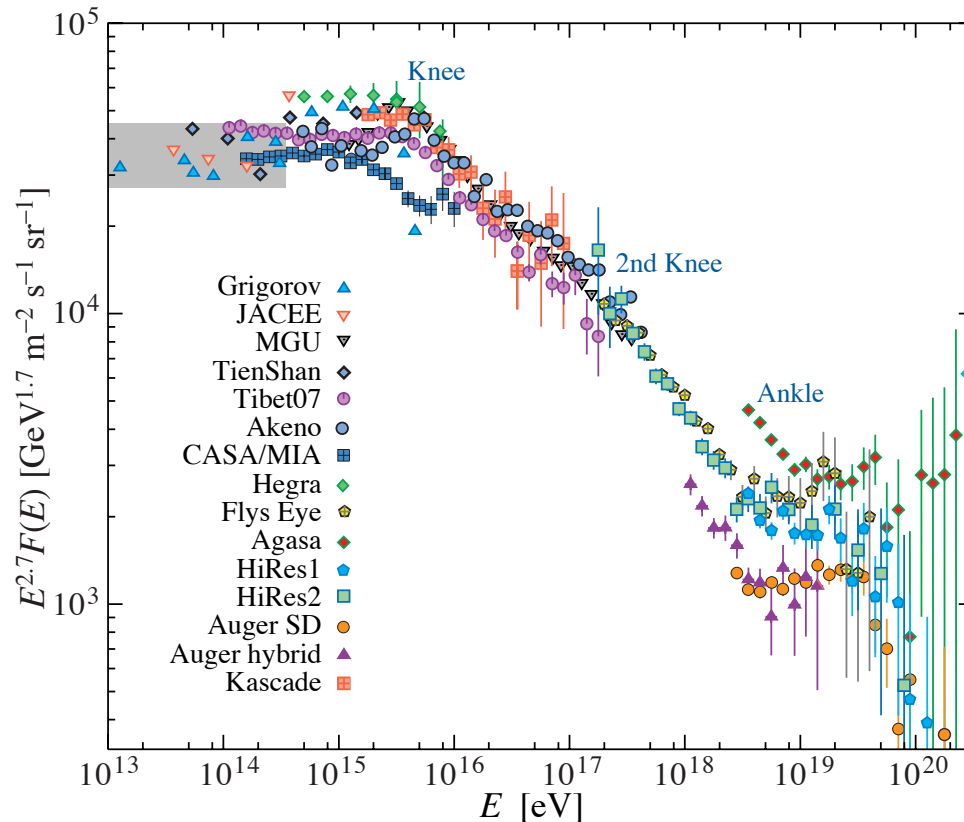
Figure 24.9: The all-particle spectrum from air shower measurements. The shaded area shows the range of the direct cosmic ray spectrum measurements. See full-color version on color pages at end of book.
