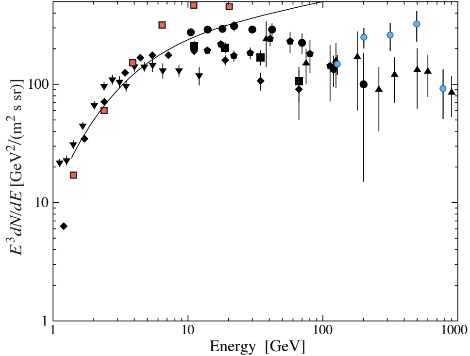
Figure 24.2: Differential spectrum of electrons plus positrons multiplied by E^3 (data from [15–22]). The line shows the proton spectrum multiplied by 0.01. See full-color version on color pages at end of book.
