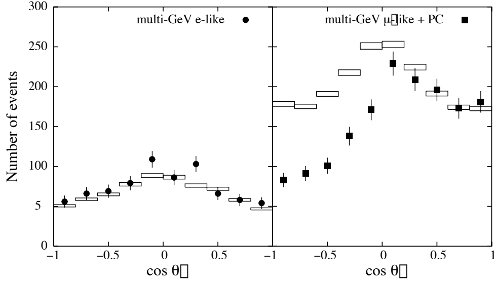
Figure 24.8: Zenith-angle dependence of multi-GeV neutrino interactions from SuperKamiokande [63]. The shaded boxes show the expectation in the absence of any oscillations.
