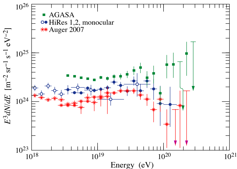
Figure 24.10: Expanded view of the highest energy portion of the cosmic-ray spectrum. ■ [86] (AGASA), ○● [87] (HiRes1,2 monocular), * [88, 89] (Auger). See full-color version on color pages at end of book.
