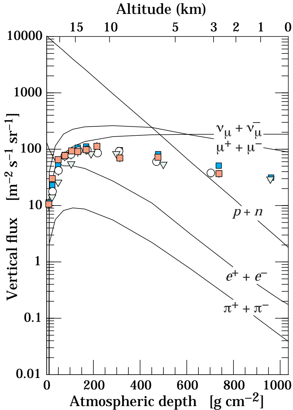
Figure 24.3: Vertical fluxes of cosmic rays in the atmosphere with E > 1 GeV estimated from the nucleon flux of Eq. (24.2). The points show measurements of negative muons with E_\mu > 1 GeV [29–32]. See full-color version on color pages at end of book.
