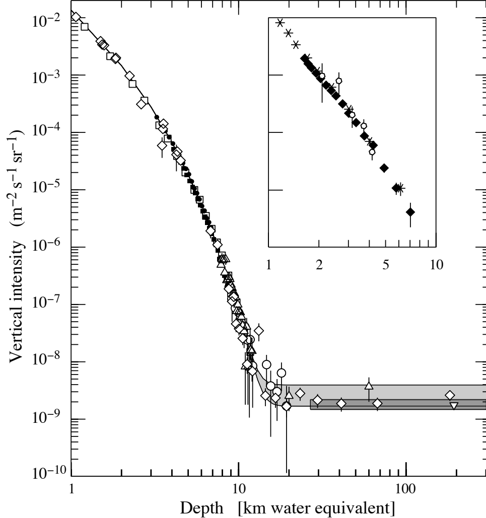
Figure 24.6: Vertical muon intensity vs depth (1 km.w.e. = 10^5 g cm ^{-2} of standard rock). The experimental data are from: \diamond : the compilations of Crouch [54], \square : Baksan [58], \circ : LVD [59], \bullet : MACRO [60], \blacksquare : Frejus [61], and \triangle SNO [62]. The shaded area at large depths represents neutrino-induced muons of energy above 2 GeV. The upper line is for horizontal neutrino-induced muons, the lower one for vertically upward muons.
