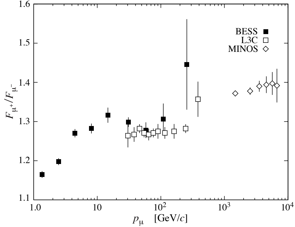
Figure 24.5: Muon charge ratio as a function of the muon momentum from Refs. [40,41,47].
