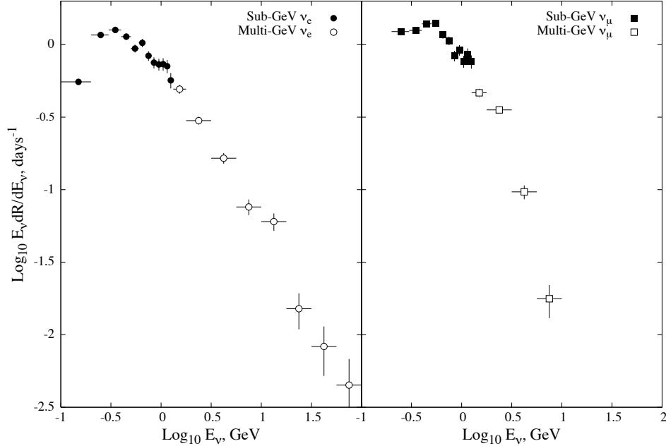
Figure 24.7: Sub-GeV and multi-GeV neutrino interactions from SuperKamiokande [63]. The plot shows the spectra of visible energy in the detector.
