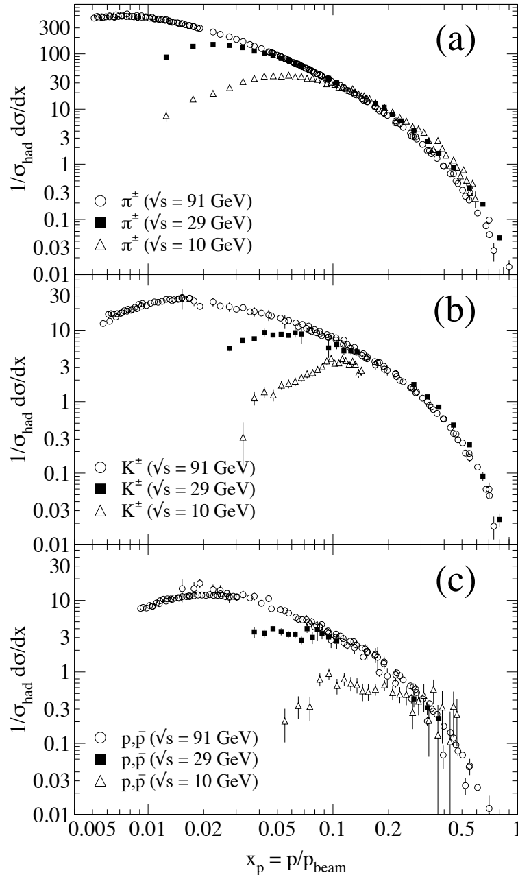
Figure 17.7: Scaled momentum spectra of (a) \pi^\pm , (b) K^\pm , and (c) p/\bar{p} at \sqrt{s} = 10, 29, \text{ and } 91 GeV are shown [22,25,55,86].
