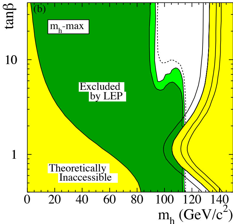
Figure 4: The MSSM exclusion limits, at 95% CL (light-green) and 99.7% CL (dark-green), obtained by LEP for the -max benchmark scenario, with m_t = 174.3 GeV. The figure shows the excluded and theoretically inaccessible regions in the (m_{h_0}, \tan \beta) projection. The upper edge of the parameter space is sensitive to the top quark mass; it is indicated, from left to right, for m_t = 169.3, 174.3, 179.3 and 183.0 GeV. The dashed lines indicate the boundaries of the regions which are expected to be excluded on the basis of Monte Carlo simulations with no signal (from Ref. [36]).
