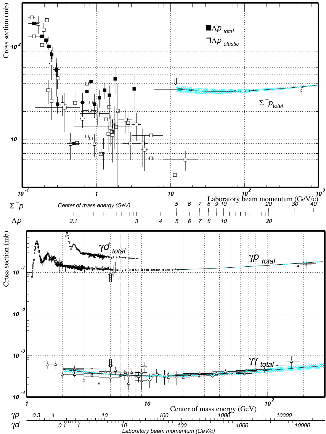
Figure 39.17: Total and elastic cross sections for \Lambda p , total cross section for \Sigma^- p , and total hadronic cross sections for \gamma d , \gamma p , and \gamma\gamma collisions as a function of laboratory beam momentum and the total center-of-mass energy. Corresponding computer-readable data files may be found at http://pdg.lbl.gov/xsect/contents.html (Courtesy of the COMPAS group, IHEP, Protvino, Russia, August 2001.)
