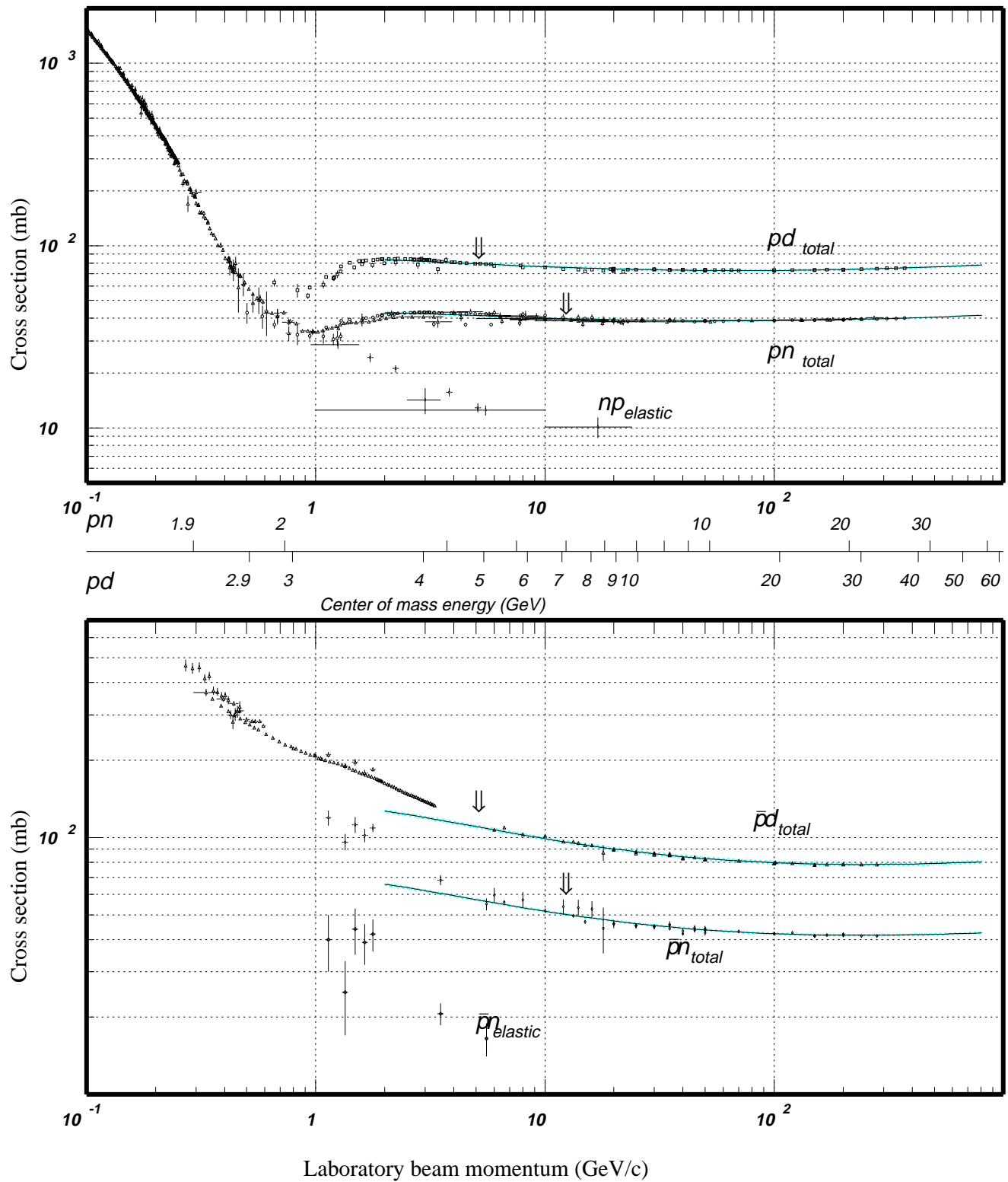
Figure 39.13: Total and elastic cross sections for pd (total only), np , \bar{p}d (total only), and \bar{p}n collisions as a function of laboratory beam momentum and total center-of-mass energy. Corresponding computer-readable data files may be found at http://pdg.lbl.gov/xsect/contents.html (Courtesy of the COMPAS Group, IHEP, Protvino, Russia, August 2001.)
