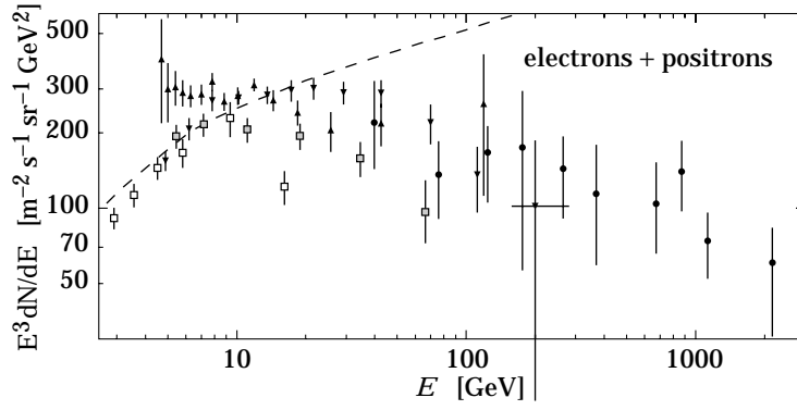
Figure 23.2: Differential spectrum of electrons plus positrons multiplied by E^3 (data summary from Ref. 8). The dashed line shows the proton spectrum multiplied by 0.01.
