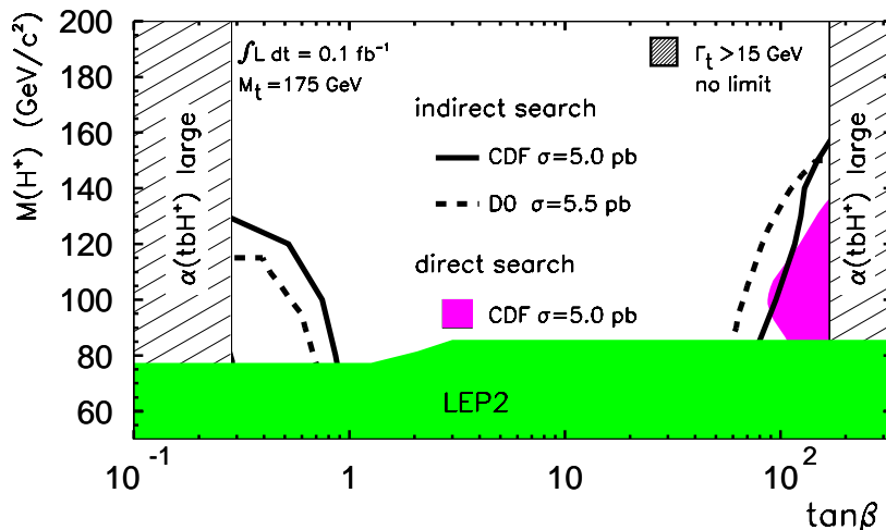
Figure 8: Summary of the 95% CL exclusions in the (m_{H^+}, \tan\beta) plane obtained by the DØ [42] and CDF [43] collaborations, using various indirect and direct observation techniques. The limits quoted by the two collaborations were obtained assuming slightly different t\bar{t} cross sections and using different statistical procedures. The LEP limits from Fig. 7 are also reproduced.
