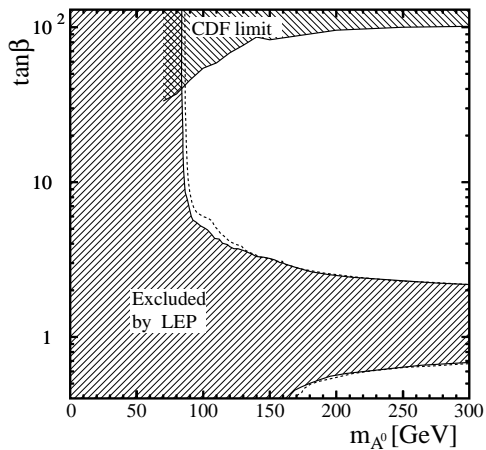
Figure 6: The 95% CL bounds on m_{h^0} , m_{A^0} , and \tan\beta , for the case of large mixing, from combining the data of the four LEP experiments up to \sqrt{s} = 196 GeV [29]. The dashed lines indicate the expected limits. The exclusions at large \tan\beta from the CDF experiment [33] are also indicated.
