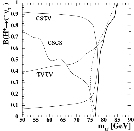
Figure 7: The 95% CL bounds on m_{H^\pm} as a function of the branching ratio B(H^+ \rightarrow \tau^+ \nu_\tau) , from combining the data collected by the LEP experiments at energies up to 196 GeV [29]. The expected exclusion limit is indicated by the dashed line and the observed limits, channel-by-channel (light) and total (heavy), by the full lines.
