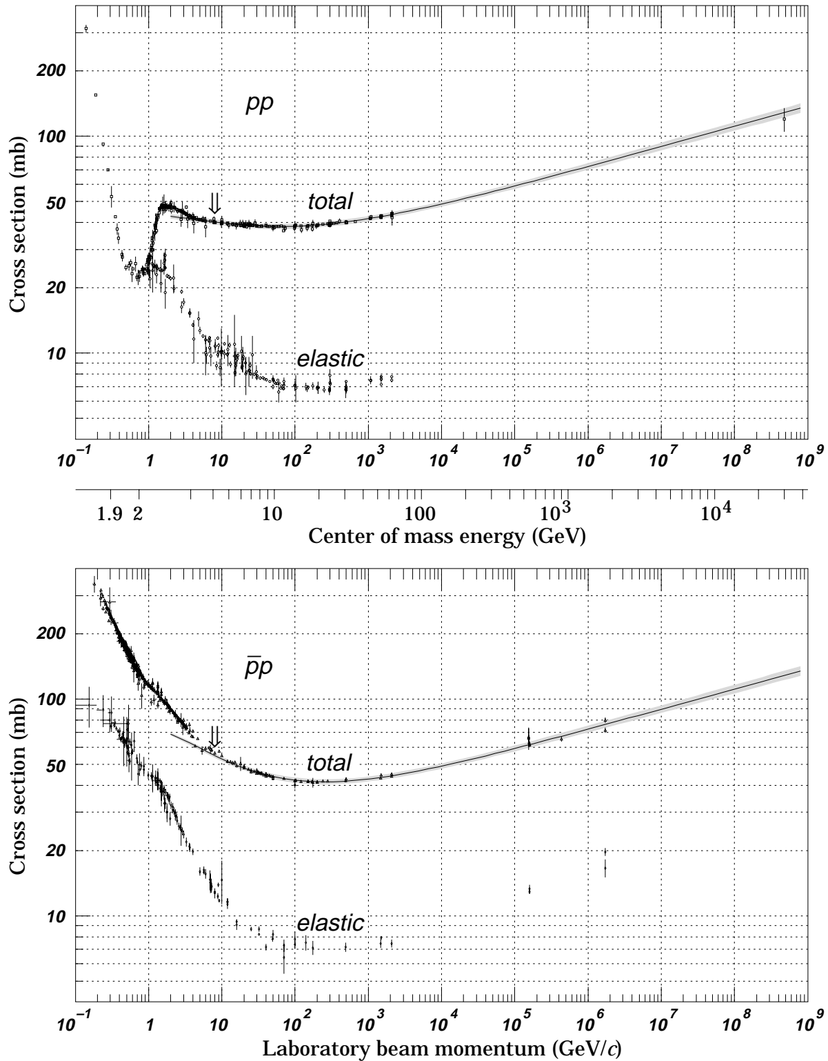
Figure 38.9: Total and elastic cross sections for pp and \bar{p}p collisions as a function of laboratory beam momentum and total center-of-mass energy. Corresponding computer-readable data files may be found at http://pdg.lbl.gov/xsect/contents.html (Courtesy of the COMPAS Group, IHEP, Protvino, Russia, August 1999.)
