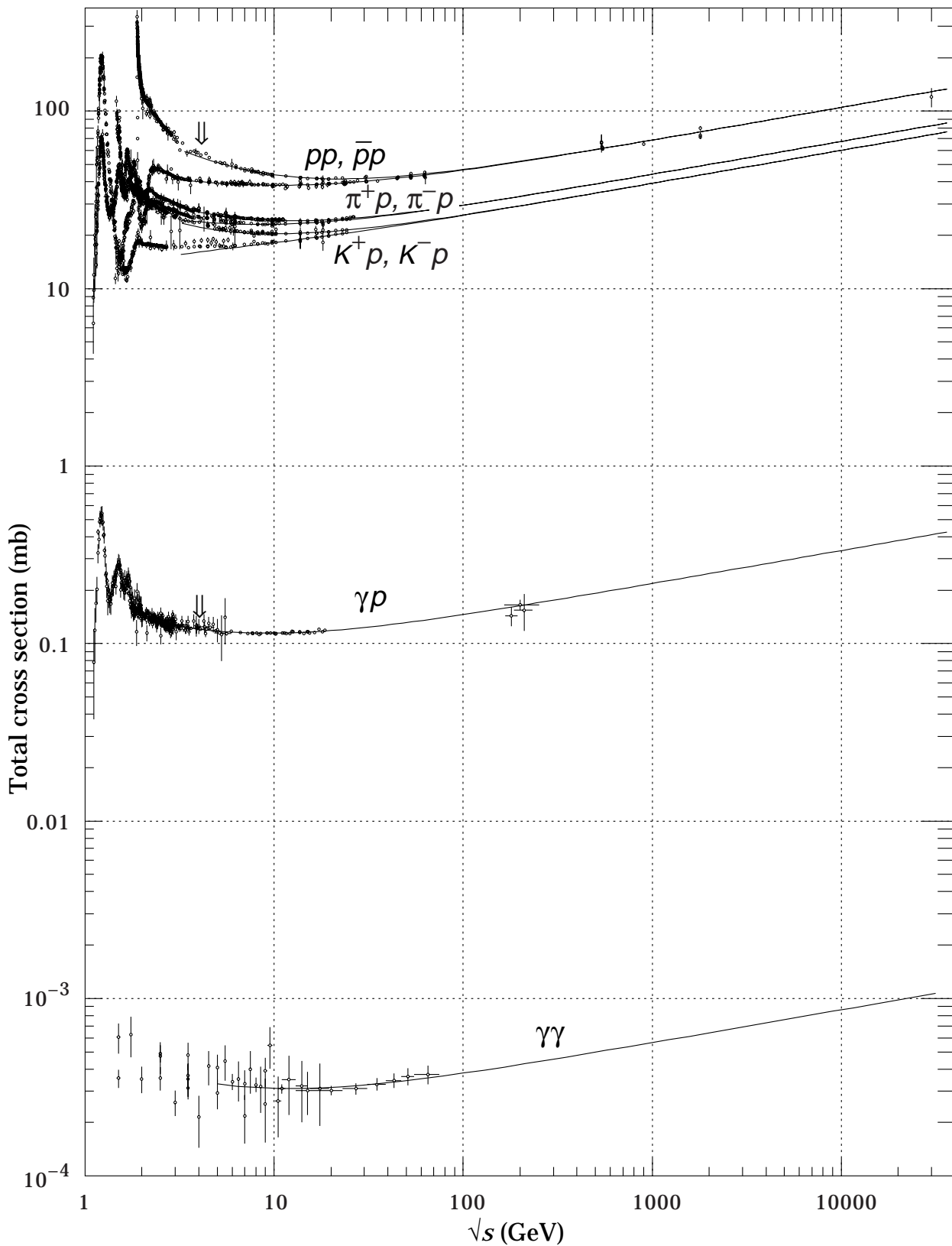
Figure 38.8: Summary of hadronic, \gamma p , and \gamma\gamma total cross sections. Corresponding computer-readable data files may be found at http://pdg.lbl.gov/xsect/contents.html (Courtesy of the COMPAS group, IHEP, Protvino, Russia, August 1999.)
