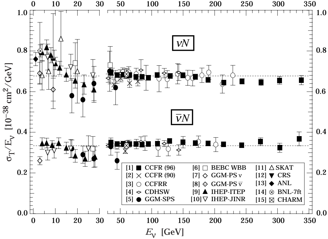
Figure 38.7: \sigma_T/E_\nu , for the muon neutrino and anti-neutrino charged-current total cross section as a function of neutrino energy. The error bars include both statistical and systematic errors. The straight lines are the averaged values over all energies as measured by the experiments in Refs. [1–4]: = 0.677 \pm 0.014 ( 0.334 \pm 0.008 ) \times 10^{-38} cm 2 /GeV. Note the change in the energy scale at 30 GeV. (Courtesy W. Seligman and M.H. Shaevitz, Columbia University, 2001.)
