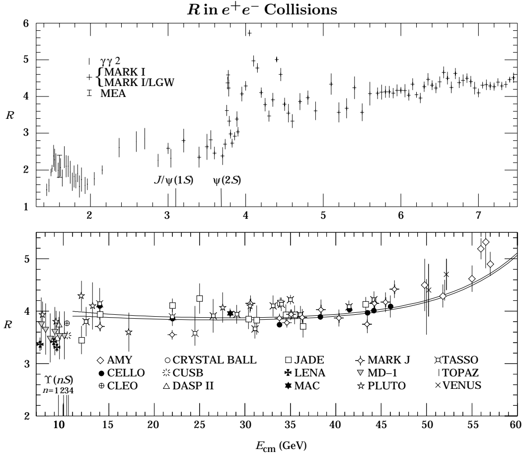
Figure 38.6: Selected measurements of R \equiv \sigma(e^+e^- \rightarrow \text{hadrons})/\sigma(e^+e^- \rightarrow \mu^+\mu^-) , where the annihilation in the numerator proceeds via one photon or via the Z . Measurements in the vicinity of the Z mass are shown in the following figure. The denominator is the calculated QED single-photon process; see the section on Cross-Section Formulae for Specific Processes. Radiative corrections and, where important, corrections for two-photon processes and \tau production have been made. Note that the ADONE data ( \gamma\gamma 2 and MEA) is for \geq 3 hadrons. The points in the \psi(3770) region are from the MARK I—Lead Glass Wall experiment. To preserve clarity only a representative subset of the available measurements is shown—references to additional data are included below. Also for clarity, some points have been combined or shifted slightly ( < 4\% ) in E_{\text{cm}} , and some points with low statistical significance have been omitted. Systematic normalization errors are not included; they range from \sim 5 – 20\% , depending on experiment. We caution that especially the older experiments tend to have large normalization uncertainties. Note the suppressed zero. The horizontal extent of the plot symbols has no significance. The positions of the J/\psi(1S) , \psi(2S) , and the four lowest \Upsilon vector-meson resonances are indicated. Two curves are overlaid for E_{\text{cm}} > 11 GeV, showing the theoretical prediction for R , including higher order QCD [M. Dine and J. Sapirstein, Phys. Rev. Lett. 43 , 668 (1979)] and electroweak corrections. The \Lambda values are for 5 flavors in the \overline{\text{MS}} scheme and are \Lambda_{\overline{\text{MS}}}^{(5)} = 60 MeV (lower curve) and \Lambda_{\overline{\text{MS}}}^{(5)} = 250 MeV (upper curve). (Courtesy of F. Porter, 1992.) References (including several references to data not appearing in the figure and some references to preliminary data):
