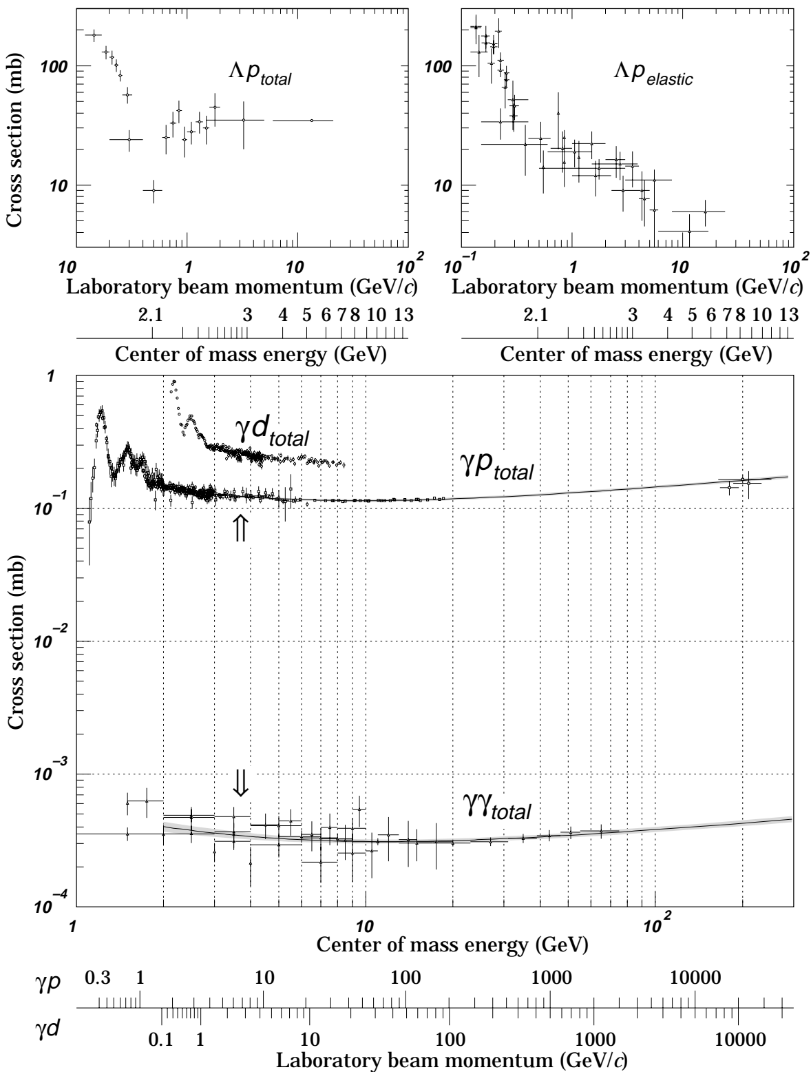
Figure 38.14: Total and elastic cross sections for \Lambda p and total hadronic cross sections for \gamma d , \gamma p , and \gamma\gamma collisions as a function of laboratory beam momentum and the total center-of-mass energy. Corresponding computer-readable data files may be found at http://pdg.lbl.gov/xsect/contents.html (Courtesy of the COMPAS group, IHEP, Protvino, Russia, August 1999.)
