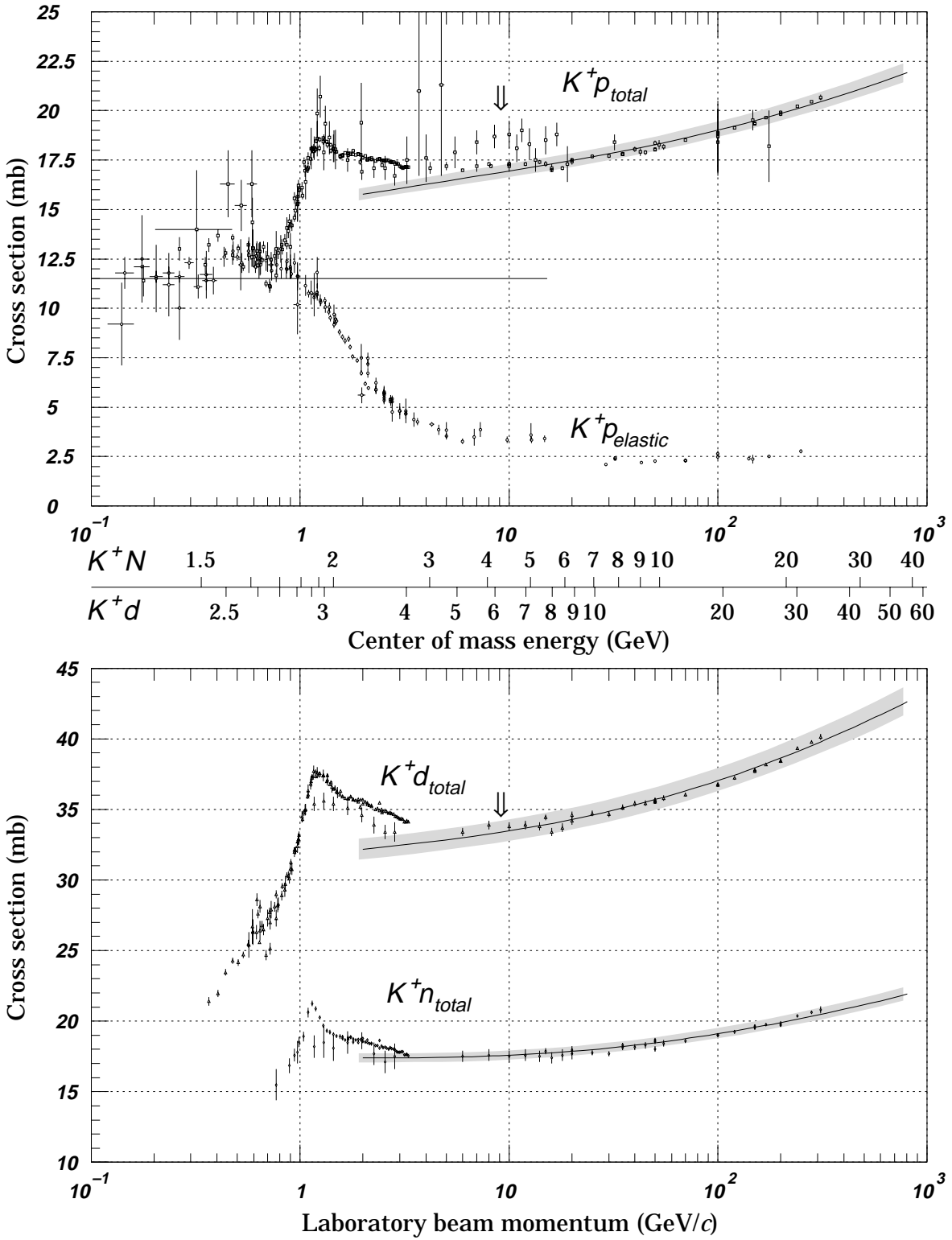
Figure 38.13: Total and elastic cross sections for K^+p and total cross sections for K^+d and K^+n collisions as a function of laboratory beam momentum and total center-of-mass energy. Corresponding computer-readable data files may be found at http://pdg.lbl.gov/xsect/contents.html (Courtesy of the COMPAS Group, IHEP, Protvino, Russia, August 1999.)
