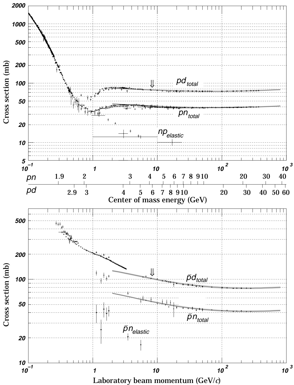
Figure 38.10: Total and elastic cross sections for pd (total only), np , \bar{p}d (total only), and \bar{p}n collisions as a function of laboratory beam momentum and total center-of-mass energy. Corresponding computer-readable data files may be found at http://pdg.lbl.gov/xsect/contents.html (Courtesy of the COMPAS Group, IHEP, Protvino, Russia, August 1999.)
