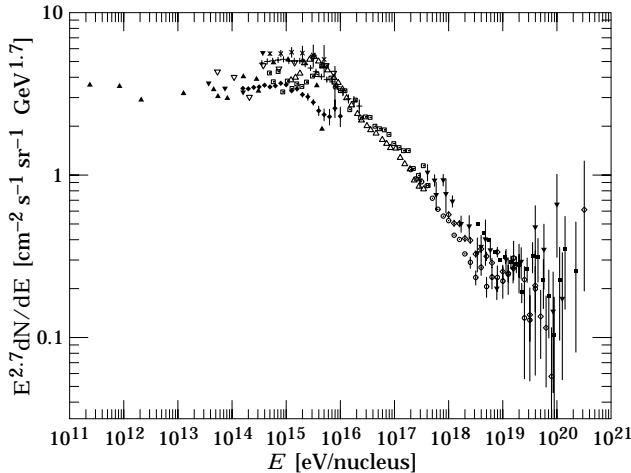
Figure 20.9: The all-particle spectrum: \square [52], \blacktriangle [54], \blacktriangledown [55], \triangle [56], \Delta [57], + [58], \times [59], \blacklozenge [60]. References for the high energy portion of the spectrum are given in Fig. 20.10.
