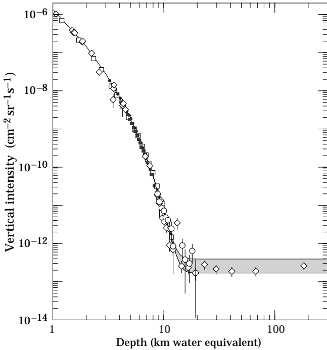
Figure 20.5: Vertical muon intensity vs depth (1 km.w.e. = 10^5 g \text{cm}^{-2} of standard rock). The experimental data are from: \diamond : the compilations of Crouch [32], \square : Baksan [33], \circ : LVD [34], \bullet : MACRO [35], \blacksquare : Frejus [36]. The shaded area at large depths represents neutrino induced muons of energy above 2 GeV. The upper line is for horizontal neutrino-induced muons, the lower one for vertically upward muons.
