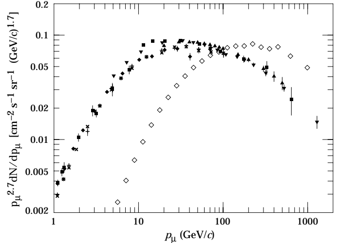
Figure 20.4: Spectrum of muons at \theta = 0^\circ ( \diamond [18], \blacksquare [20], \blacktriangledown [21], \blacktriangle [22], \times , + [23]), and \theta = 75^\circ ( \diamond [24]).
