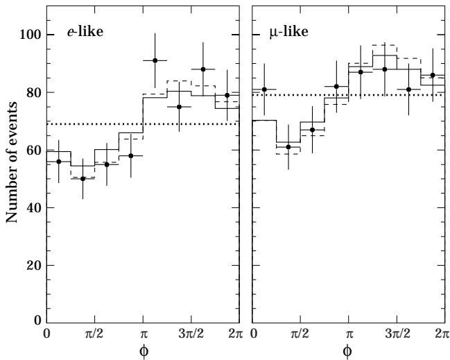
Figure 20.8: Azimuthal dependence of \sim GeV neutrino interactions from SuperKamiokande [44]. The cardinal points of the compass are S, E, N, W starting at 0. These are the direction from which the particles arrive. The lines show the expectation based on two different calculations, as described in Ref. 44.
