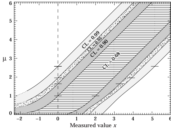
Figure 29.4: Plot of 99%, 95%, 90%, and 68.27% (“one \sigma ”) confidence intervals for a physical quantity \mu based on a Gaussian measurement x (in units of standard deviations), for the case where the true value of \mu cannot be negative. The curves become straight lines above the horizontal tick marks. The probability of obtaining an experimental value at least as negative as the left edge of the graph ( x = -2.33 ) is less than 1%. Values of x more negative than -1.64 (dotted segments) are less than 5% probable, no matter what the true value of \mu .
