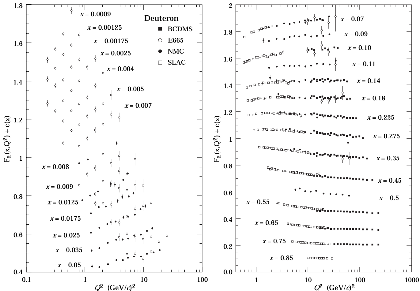
Figure 38.4: As Fig. 38.3, for the deuteron structure function F_2^d . References: BCDMS —A.C. Benvenuti et al. , Phys. Lett. B237 , 592 (1990). E665 , NMC , SLAC —same references as Fig. 38.3. (Courtesy of R. Voss, 1996.)
