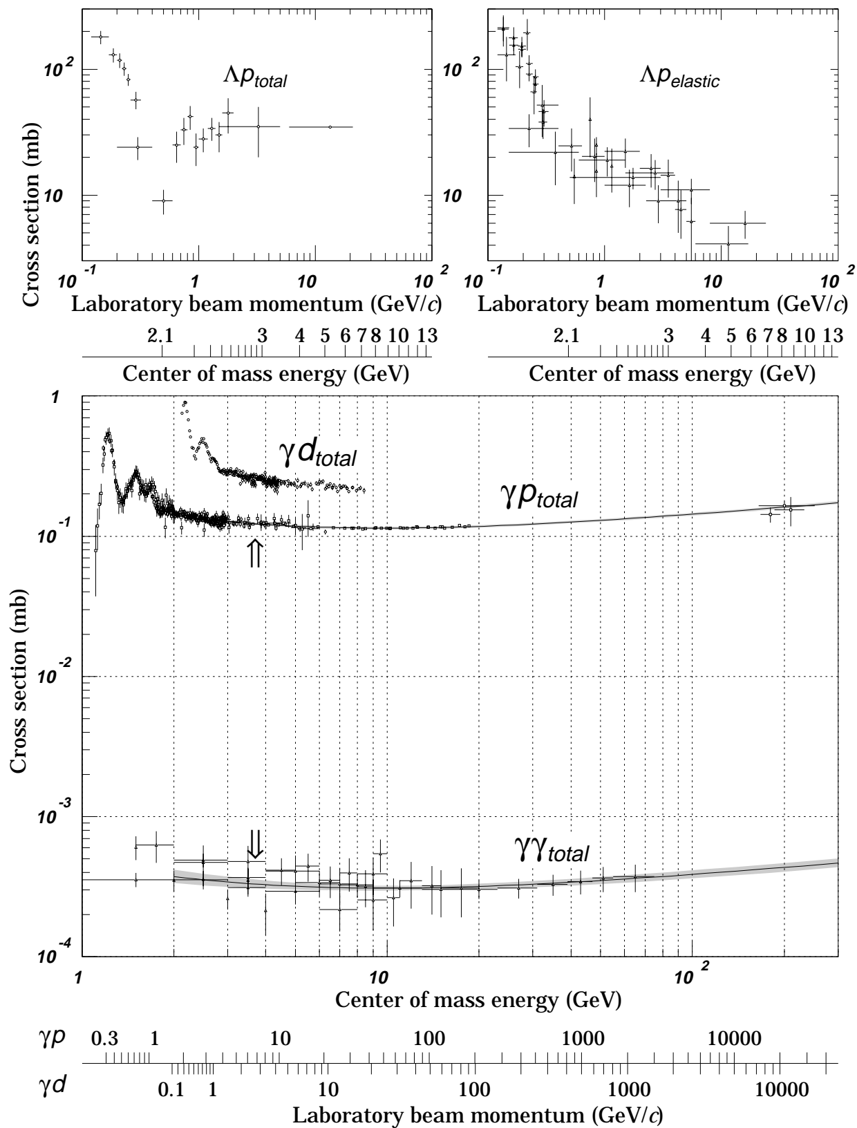
Figure 38.23: Total and elastic cross sections for \Lambda p and total hadronic cross sections for \gamma d , \gamma p , and \gamma\gamma collisions as a function of laboratory beam momentum and the total center-of-mass energy. Corresponding computer-readable data files may be found at http://pdg.lbl.gov/xsect/contents.html (Courtesy of the COMPAS group, IHEP, Protvino, Russia, April 1998.)
