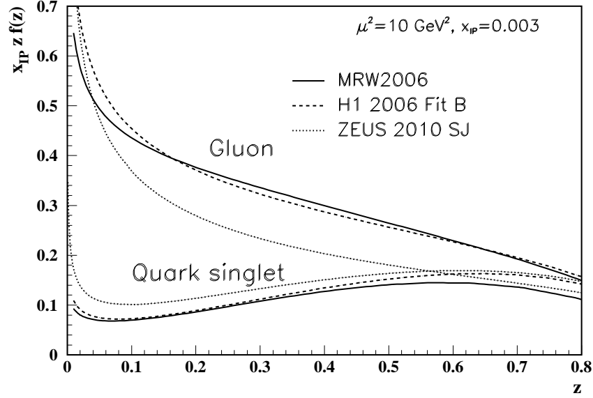
Figure 16.6: Diffractive parton distributions, x_{\mathbb{P}} z f_{a/p}^{\mathbb{D}} , obtained from fitting to the ZEUS data with Q^2 > 5 \text{ GeV}^2 [86], H1 data with Q^2 > 8.5 \text{ GeV}^2 assuming Regge factorization [81], and using a more perturbative QCD approach [87]. Only the Pomeron contributions are shown and not the secondary Reggeon contributions, which are negligible at the value of x_{\mathbb{P}} = 0.003 chosen here. The H1 2007 Jets distribution [88] is similar to H1 2006 Fit B.
