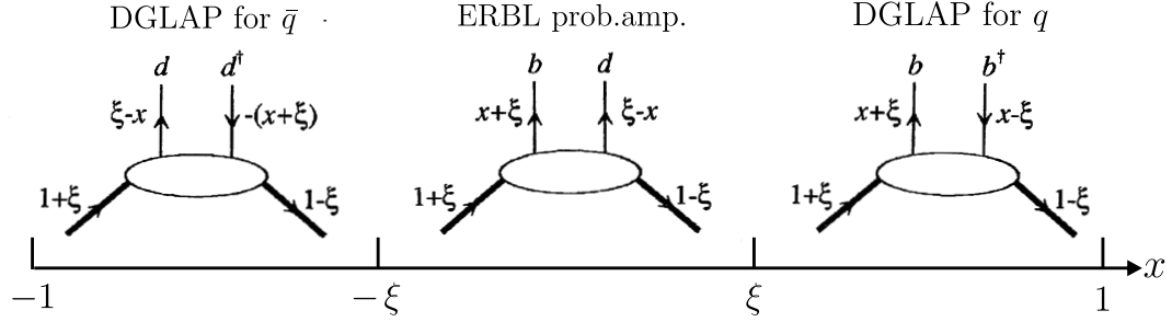
Figure 16.7: Schematic diagrams of the three distinct kinematic regions of (the imaginary part of) H_q . The proton and quark momentum fractions refer to \bar{P}^+ , and x covers the interval (-1,1) . In the ERBL domain the GPDs are generalisations of distribution amplitudes which occur in processes such as p\bar{p} \rightarrow J/\psi .
