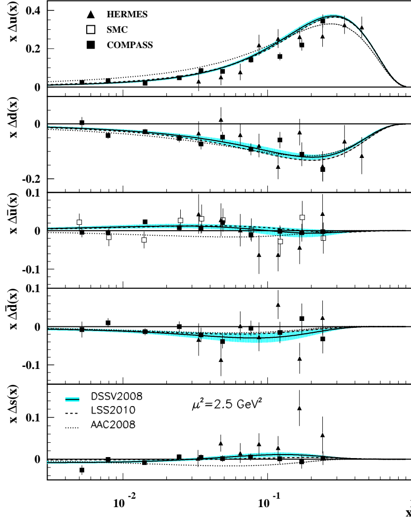
Figure 16.5: Distributions of x times the polarized parton distributions \Delta q(x) (where q = u, d, \bar{u}, \bar{d}, s ) using the LSS2010 [57], AAC2008 [54], and DSSV2008 [55] parameterizations at a scale \mu^2 = 2.5 \text{ GeV}^2 , showing the error corridor of the latter set (corresponding to a one-unit increase in \chi^2 ). See also BB2010 [56]. Points represent data from semi-inclusive positron (HERMES [61,62]) and muon (SMC [63] and COMPASS [64,65]) deep inelastic scattering given at Q^2 = 2.5 \text{ GeV}^2 . SMC results are extracted under the assumption that \Delta \bar{u}(x) = \Delta \bar{d}(x) .
